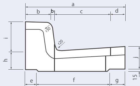
L形縁塊 (500)
